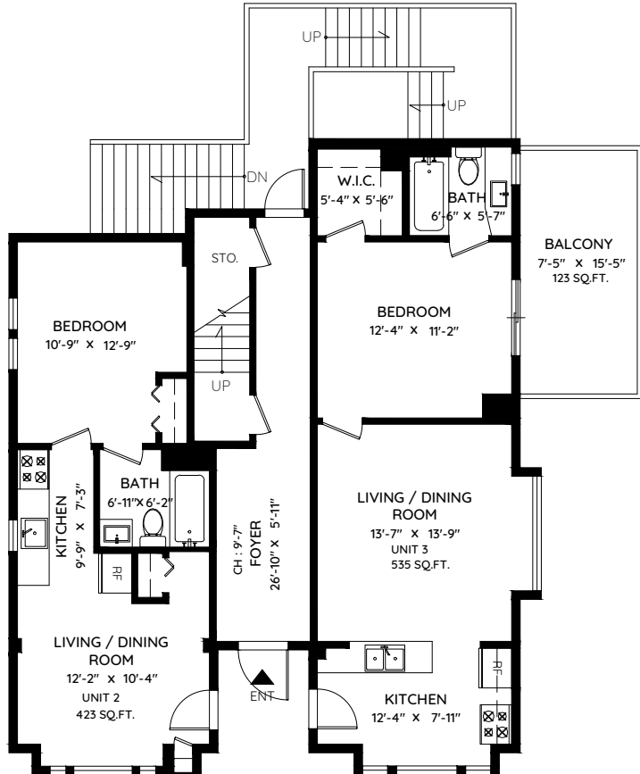
MAIN FLOOR 1,157 SQ.FT. CH: 9'-8"
